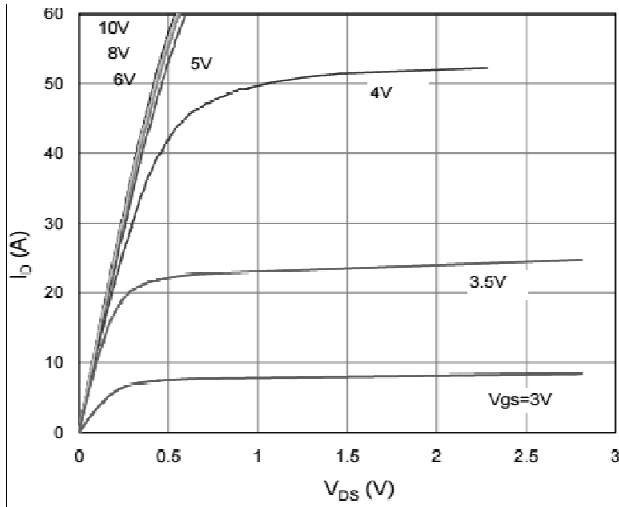
Output Characteristic
