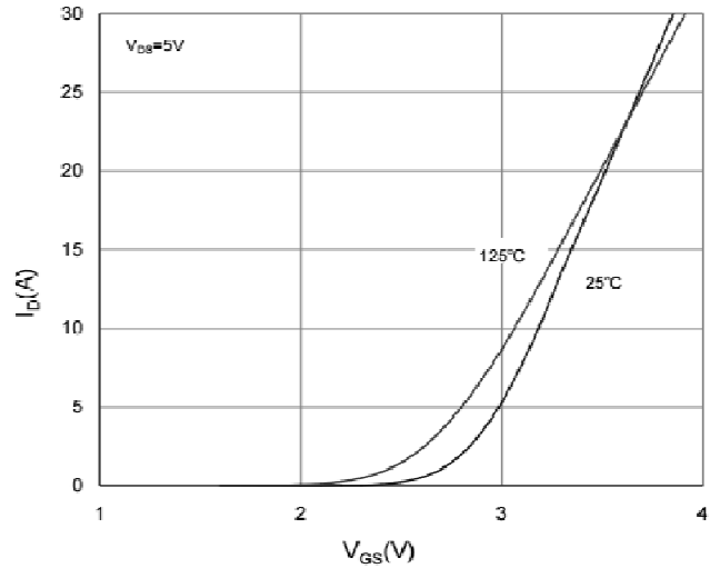
Transfer Characteristic
